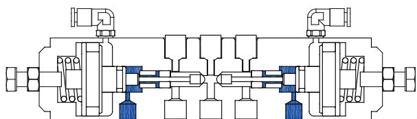
ACCV INHIBITOR FLUID FILLING CHAMBER
