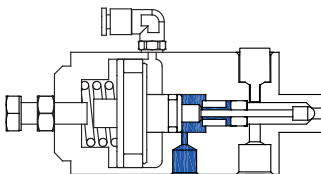
AMV INHIBITOR FLUID FILLING CHAMBER
